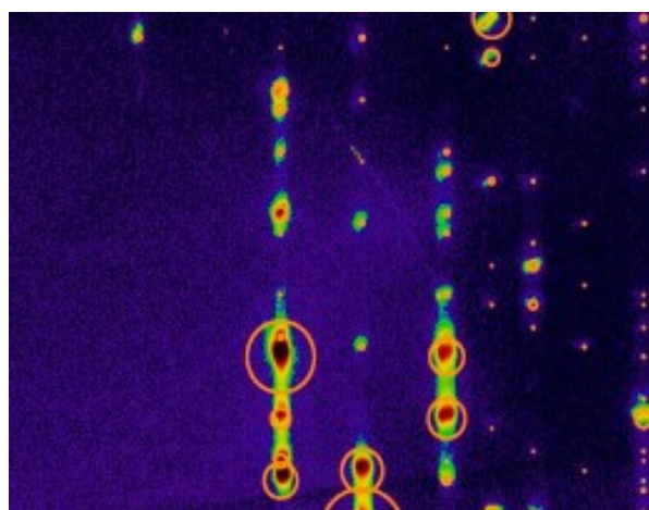
x-ray diffraction on pure 4T. Credit: HZB
